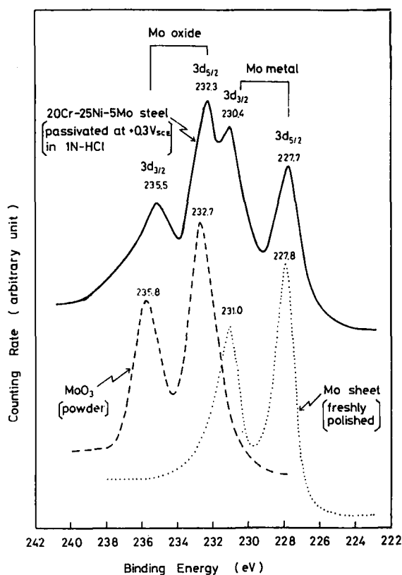
FIG. 11. Comparison of the XPS spectra of the Mo 3d 3/2 -3d 5/2 levels for the 20Cr-25Ni-5Mo steel passivated at +0.30V in 1N HCl for 1 h, MoO 3 powder, and a freshly polished sheet of metallic Mo.
